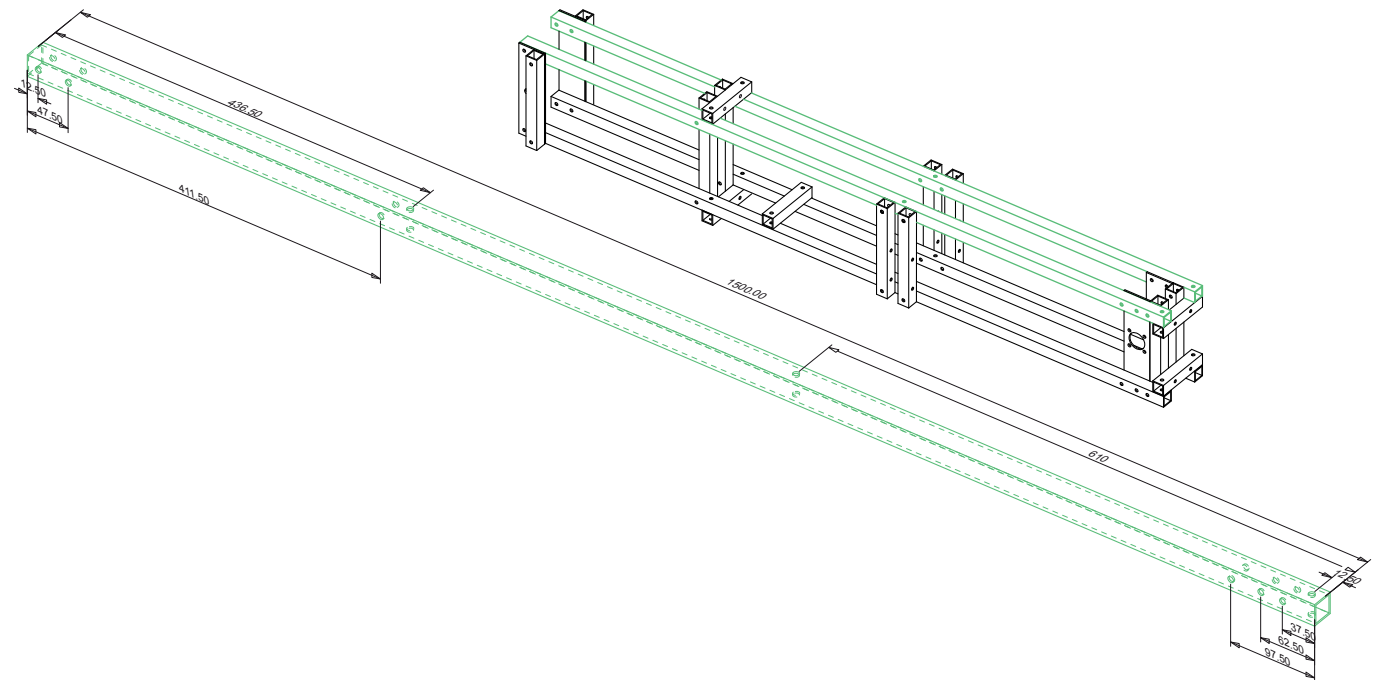
Frame component FR_1b x2 25mm square aluminium tubing 2mm material thickness 6.5mm Ø holes
