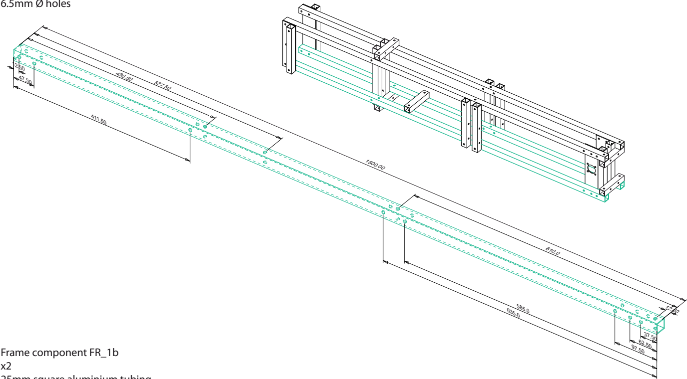
Frame component FR_1a x2 25mm square aluminium tubing 2mm material thickness 6.5mm Ø holes
